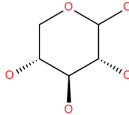
Pentopyranoses e.g. D-Xylopyranose
