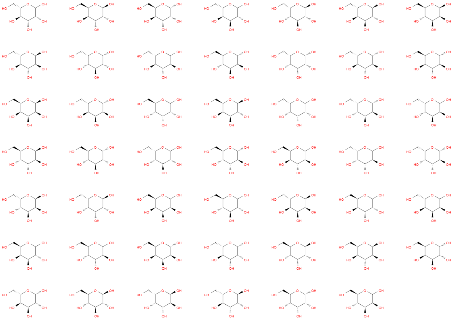
48 hexopyranoses
